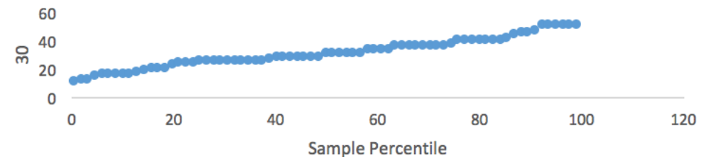
Normal Probability Plot
