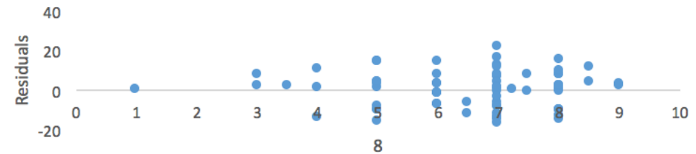
8 Residual Plot
