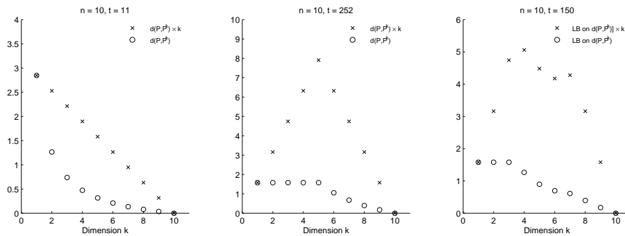
Figure 1: (a) Example 1 with n = 10 . (b) Example 2 with n = 10 . (c) Example 3.
