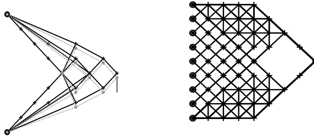
“Long-bar truss:” 38 bars, compliance 0.1914 “Short-bar truss:” 128 bars, compliance 0.2903
