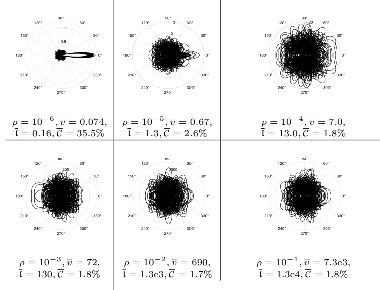
Figure S2II.2. Nominal diagram – reality, Magnitudes of 100 actual diagrams stemming from the optimal solution to (P)
