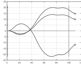
Figure S2IV.3. Coordinates of system's state vs. time. Circles: forecasts; dotted segment between dotted vertical lines: instants where observations are taken.
