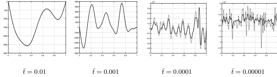
Figure S2IV.5. Sample recoveries: dotted line - true; solid line - recovery
