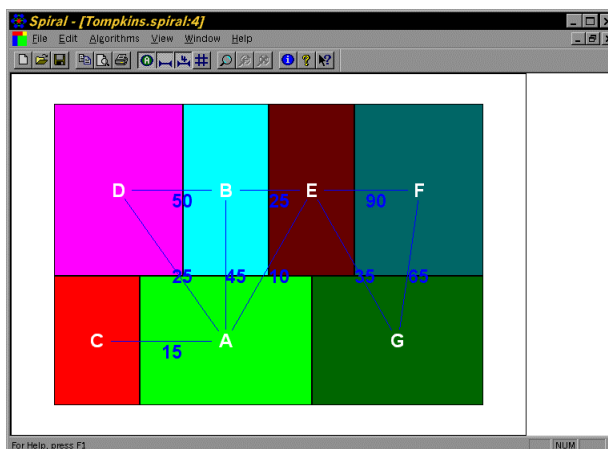
Figure 17.13. Spiral Three Exchange Layout for the Tompkins Example
