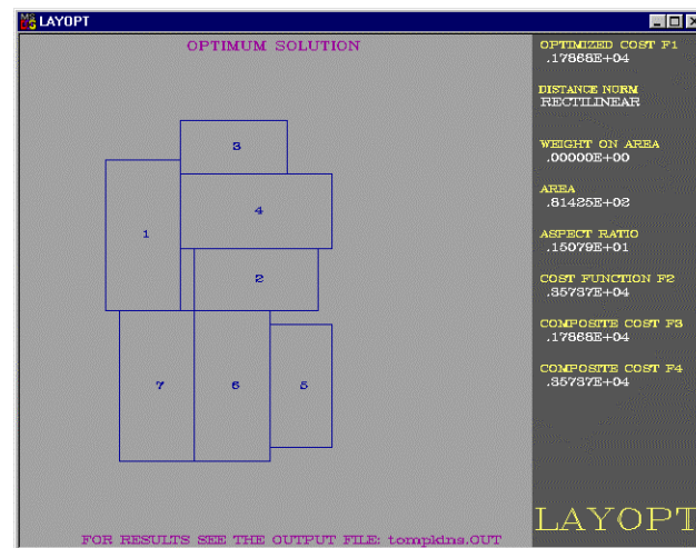
Figure 17.40. PLANOPT Layout for the Tompkins Example
