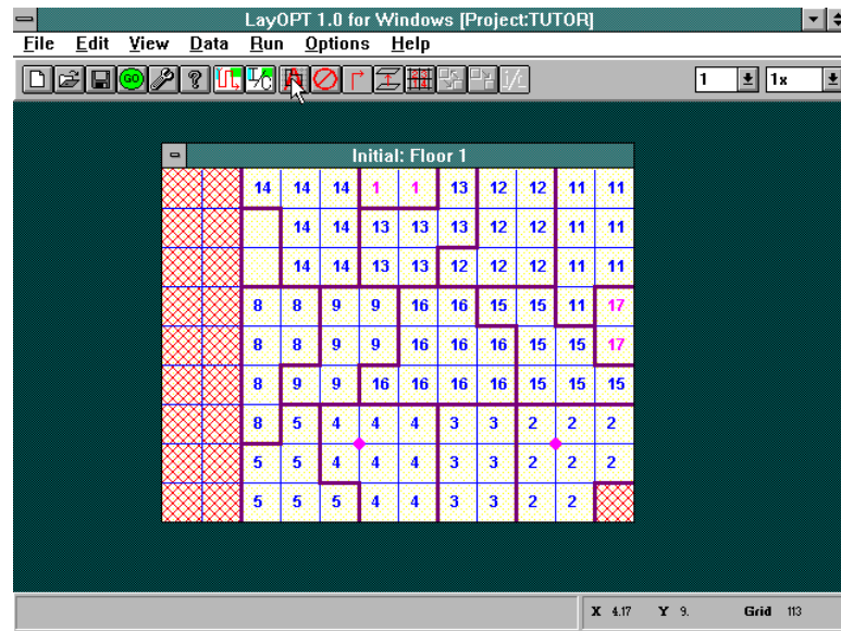
Figure 17.29. Initial LayOPT Layout
