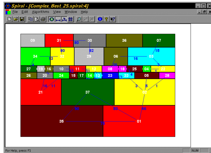
Figure 17.25. Spiral Layout for Complex Case with Maximum Shape Factor = 2.5
