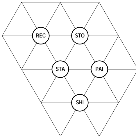
Figure 17.18. Adjacency Graph with 5 Departments for the Parts Example
