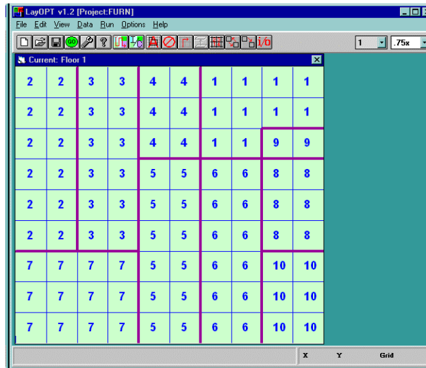
Figure 17.37. Final Layout for the Furniture Example
