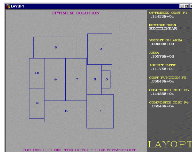
Figure 17.41. PLANOPT Layout for the Furniture Example
