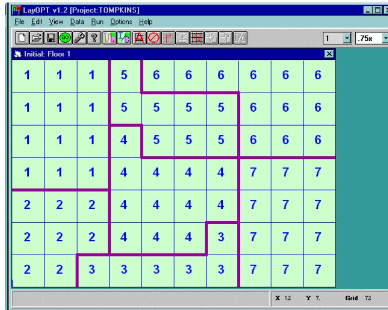
Figure 17.33. Initial Layout for the Tompkins Example
