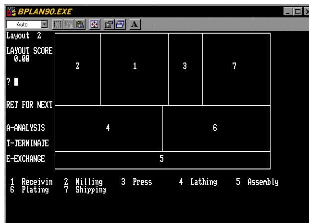
Figure 17.39. BLOCPLAN Layout for the Tompkins Example with Numerical Data
