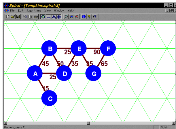
Figure 17.9. Spiral No-Exchange Graph for the Tompkins Example
