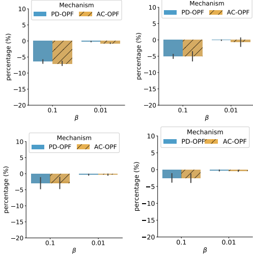
Fig. 5. Dispatch costs differences between the optimal and the PD-OPF solution (PD-OPF) and its centralized AC-OPF counterpart. IEEE 39 (top) & IEEE 57 bus (bottom), \alpha = 0.01 (left), 0.1 (right), \beta = [0.1, 0.01] .
