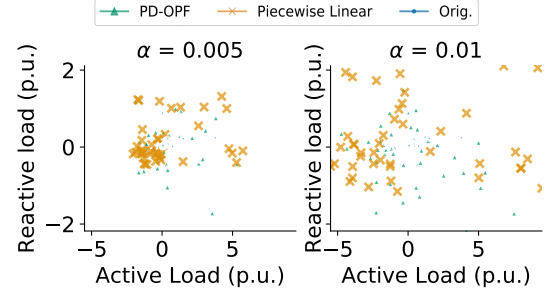
Fig. 8. Loads from the original dataset and the Piecewise Linear & ADMM Mechanisms on the IEEE-57 bus system.
