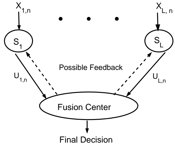
Fig. 1. General setting for decentralized decision systems
