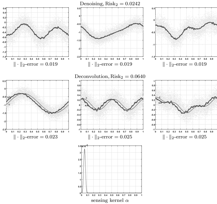
Figure 6.3: Smooth curve: f ; “bumpy” curve: recovery; gray cloud: observations. In all experiments, n = 8192 , \varkappa = 2 , p_0 = p_1 = p_2 = 2 , \sigma = 0.5 , L_t = (10\pi)^t , 0 \leq t \leq 2 .
