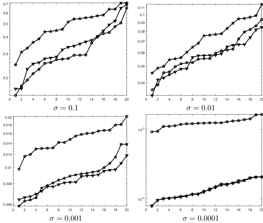
Figure 5.1: Recovery errors for the near-optimal linear estimate (circles) and for polyhedral estimates yielded by Proposition 5.8 ( PolyI , pentagrams) and by the construction from Section 5.1.4 ( PolyII , triangles), 20 simulations per each value of \sigma .
