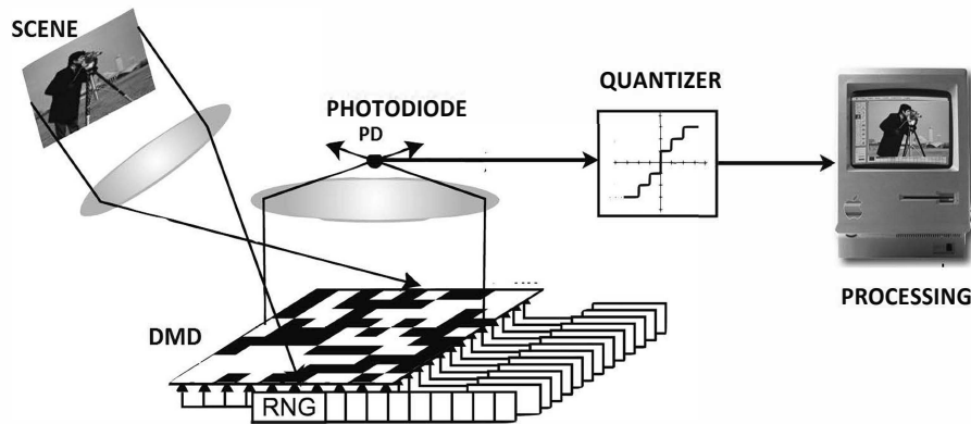
Figure 1.2: Single-pixel camera.
