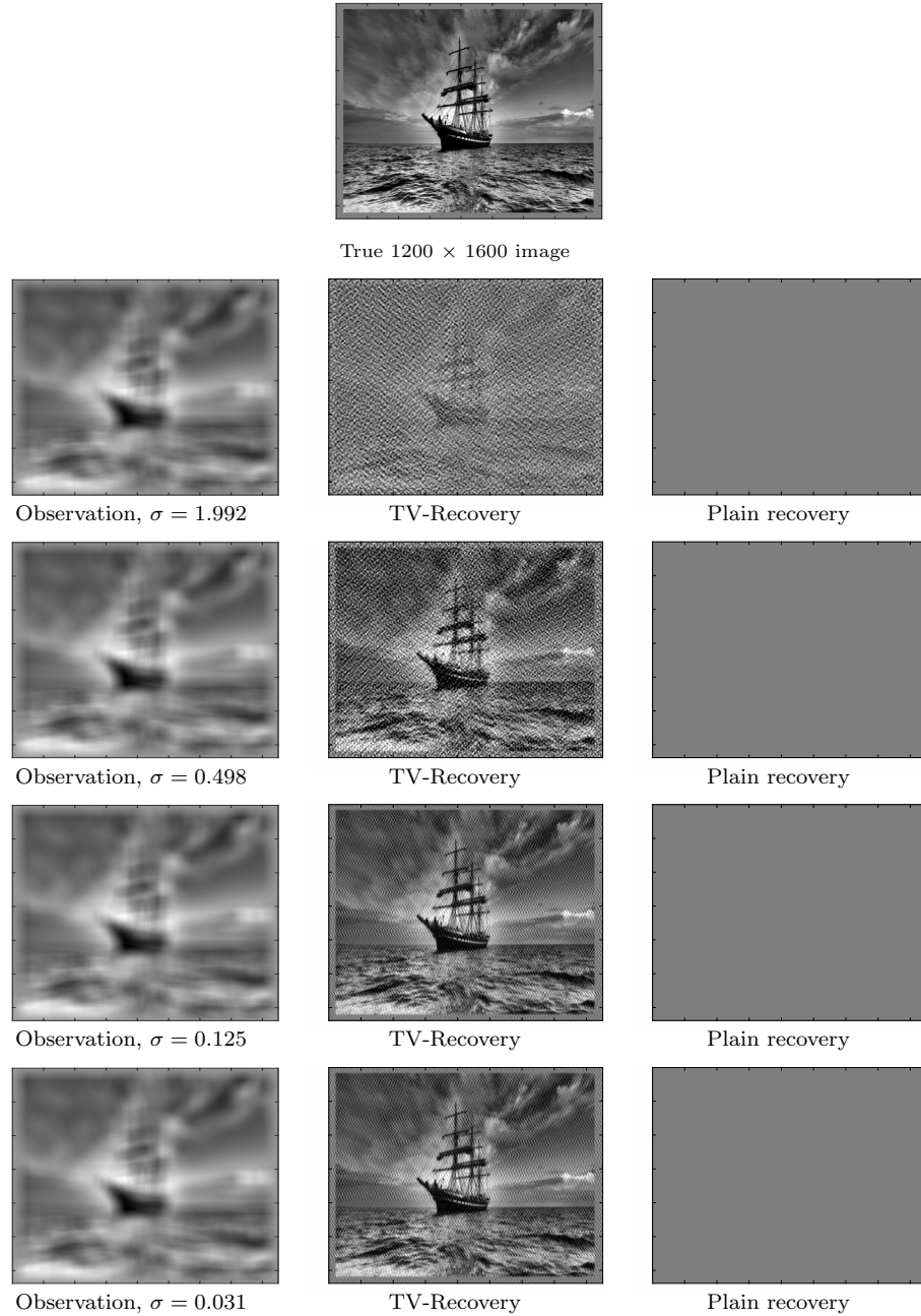
Figure 6.1: Recovery of a 1200 \times 1600 image at different noise levels, ill-posed case \Delta = 0 .
