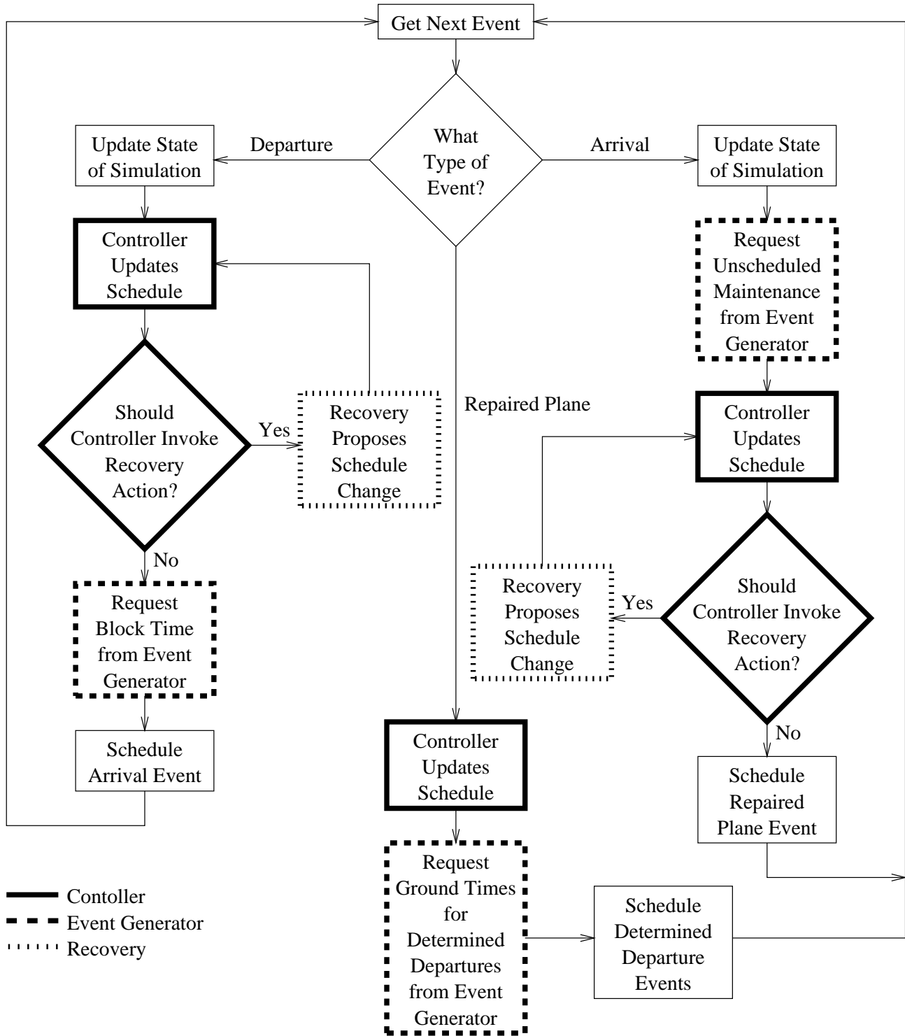
Figure 1: The Structure of SimAir
